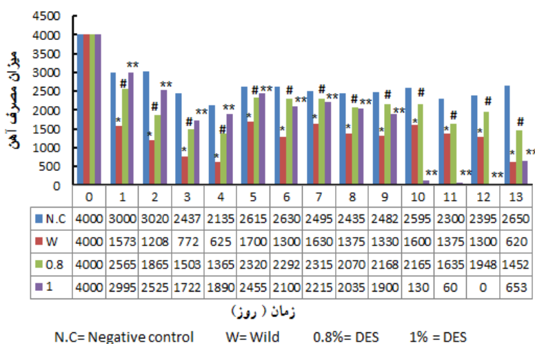
Fig. 3. Oxidation and reduction rates by wild bacteria compared with mutated bacteria by DES 0.8%, 1%. (NC: Negative Control, W: wild Bacteria, 0.8%: Mutation caused by DES 0.8% (V/V), 1%: Mutation caused by DES 1% (V/V)). The ** sign represents the result of statistical analysis Des 1% (V/V) mutant, which is significant with Wild bacteria ( P < 0.05 ).
