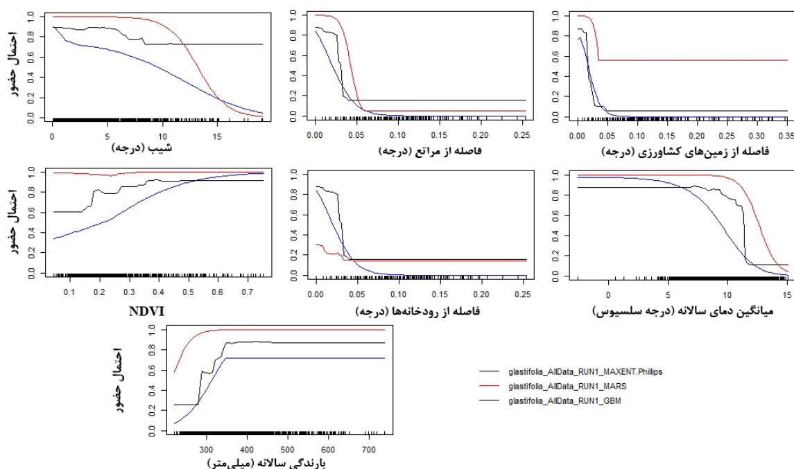
Figure 3. Response curves of Centaurea glastifolia presence to each environmental variable in each habitat distribution model (for better presentation, only one replication of three models; MaxEnt with blue line, MARS with red line and GBM with black line were presented.).
