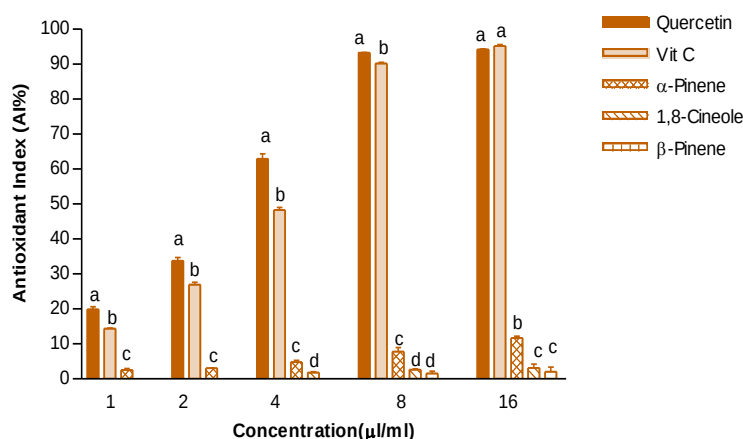
Fig. 2. Free radical-scavenging activity of α-pinene, β-pinene and 1,8-cineole in DPPH assay.
