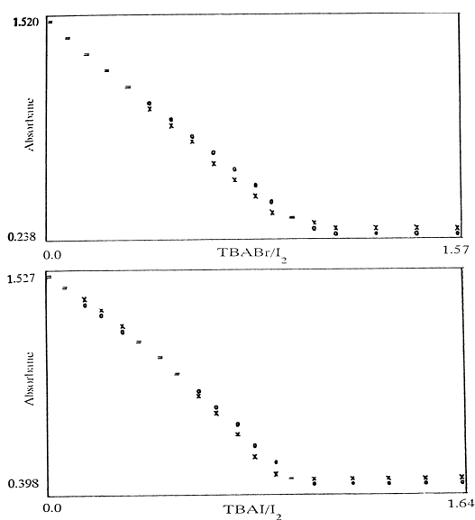
Fig.7: Plots of absorbance vs. \text{TBAX/I}_2 mole ratio for solutions of 1.65 \times 10^{-3} \text{ M} of iodine in chloroform obtained at 508nm: \text{TBAI-I}_2 ( \bullet ), \text{TBABr-I}_2 (+).
