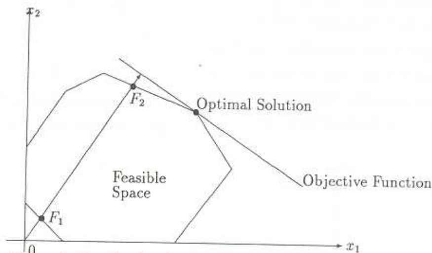
Figure 1. Combination of orthogonality and simplex method.
