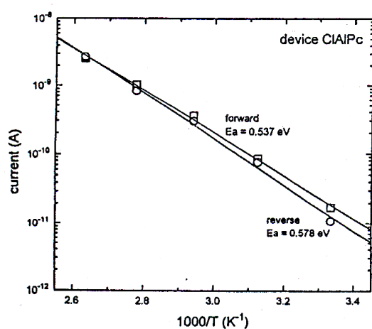
Fig. 6 (a): A semi-logarithmic plot of \log I against 1000/T For a CIAIPc device
