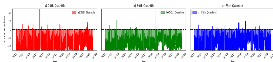
Fig. 3: Dynamic Rolling-Window NET Connectedness for SGR (100-day rolling-window, lags=1, forecast horizon=10 days)
