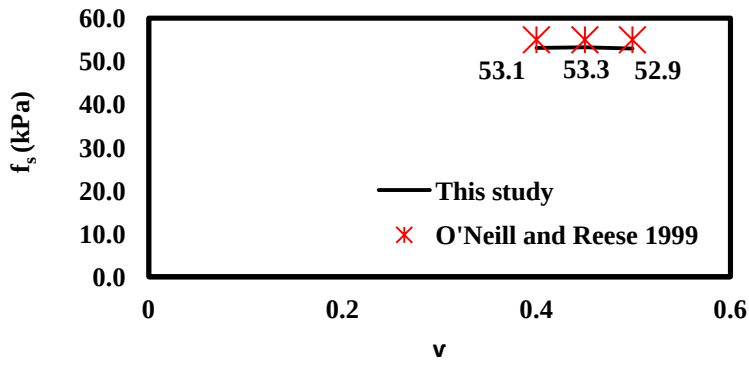
Figure 19. Effect of soil Poisson's ratio on side resistance
