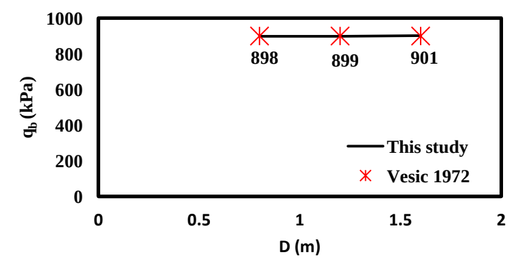
Figure 14. Effect of pile diameter on tip resistance
