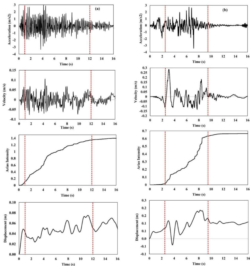
Figure 7. Comparison of the model response under the effect of (a) the near-fault ground motion (San Fernando (Pacoima Dam upper left abut)) and (b) the far-fault ground motion (San Fernando (Santa Anita Dam))
