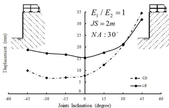
Figure 13. Effect of joints dip on cantilever displacement and lateral bulging, nail angle 30^\circ
