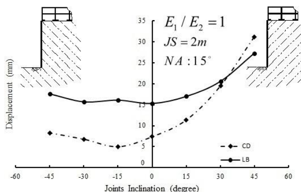
Figure 12. Effect of joints dip on cantilever displacement and lateral bulging, nail angle 15^\circ
