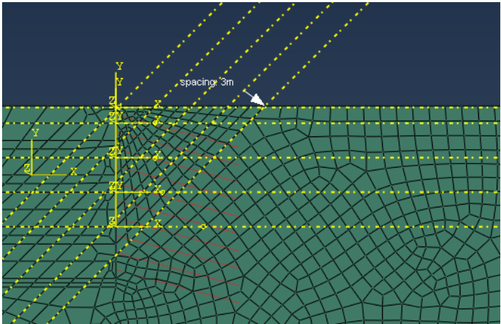
Figure 7 Developed FE model for RNW performance study Table 4. Phases of FE model staged construction
