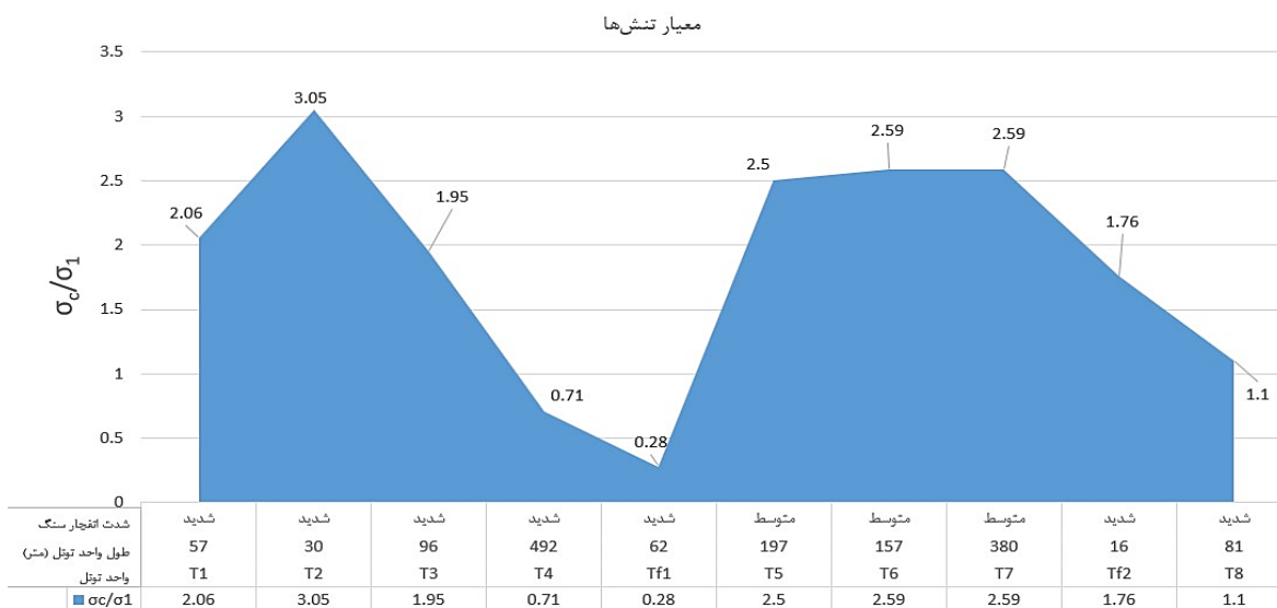
Fig. 4. Evaluation diagram of rock burst intensity based on stress criterion
