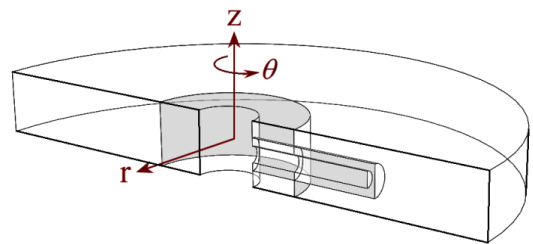
Figure 5. Typical computational domain of a half-perforation model (HPM)
