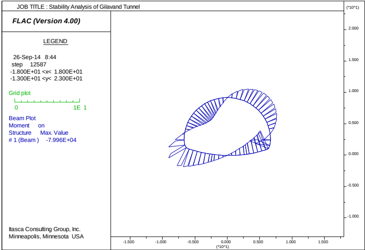
Figure3. The bending moments created in the structure after the final calculations
