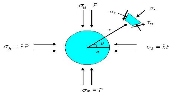
Figure 4. Stress distribution around a circle drilling
